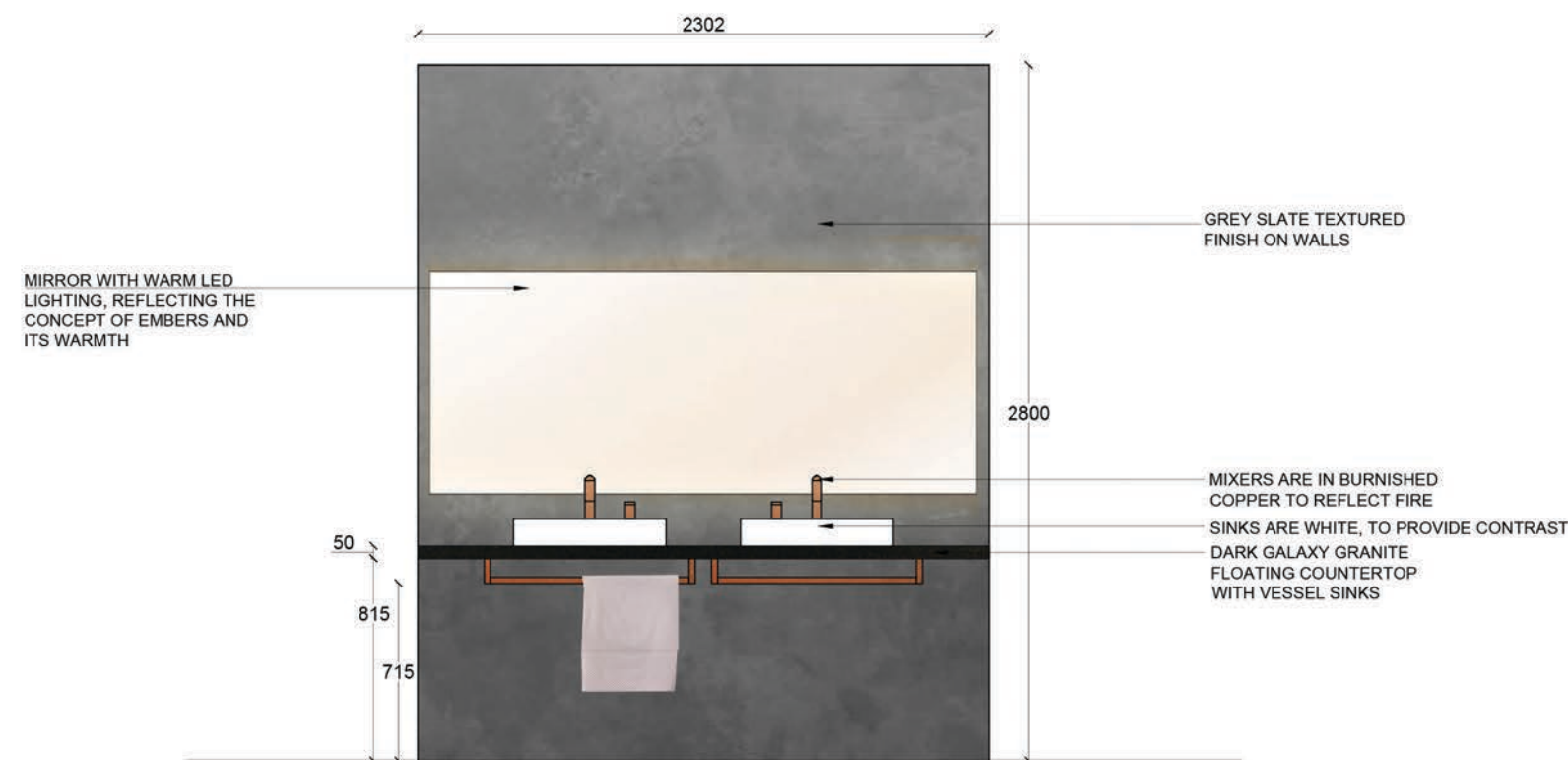
3a ELEVATION 1 SCALE 1:30
