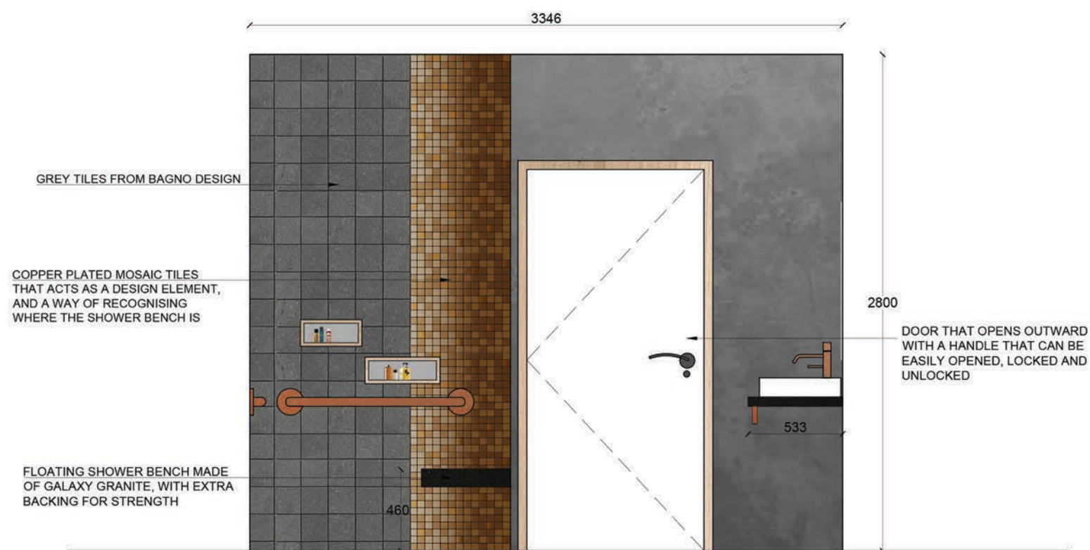
3d ELEVATION 4 SCALE 1:30
